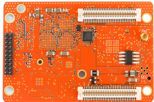
Figure 1: Pixsi Multi - Top and Bottom View
